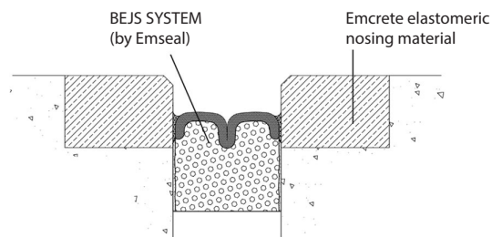
Figure 1: Emcrete Used as Expansion Joint Nosing Material
